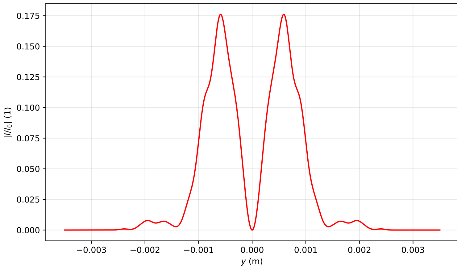
Intensity profile I(x=0, y, z=1.831)/I_0 , \text{Pin}=5.0\text{Pcr} , artificial time
